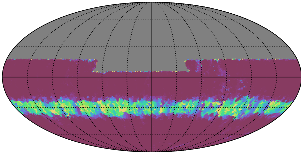
baseline_v2.0_10yrs All sky u band: Min normairmass
