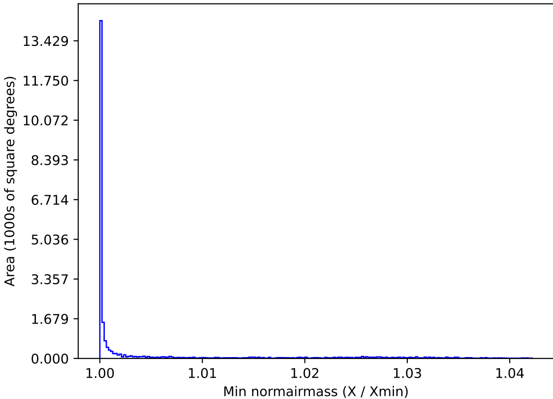
baseline_v2.0_10yrs All sky u band: Min normairmass
