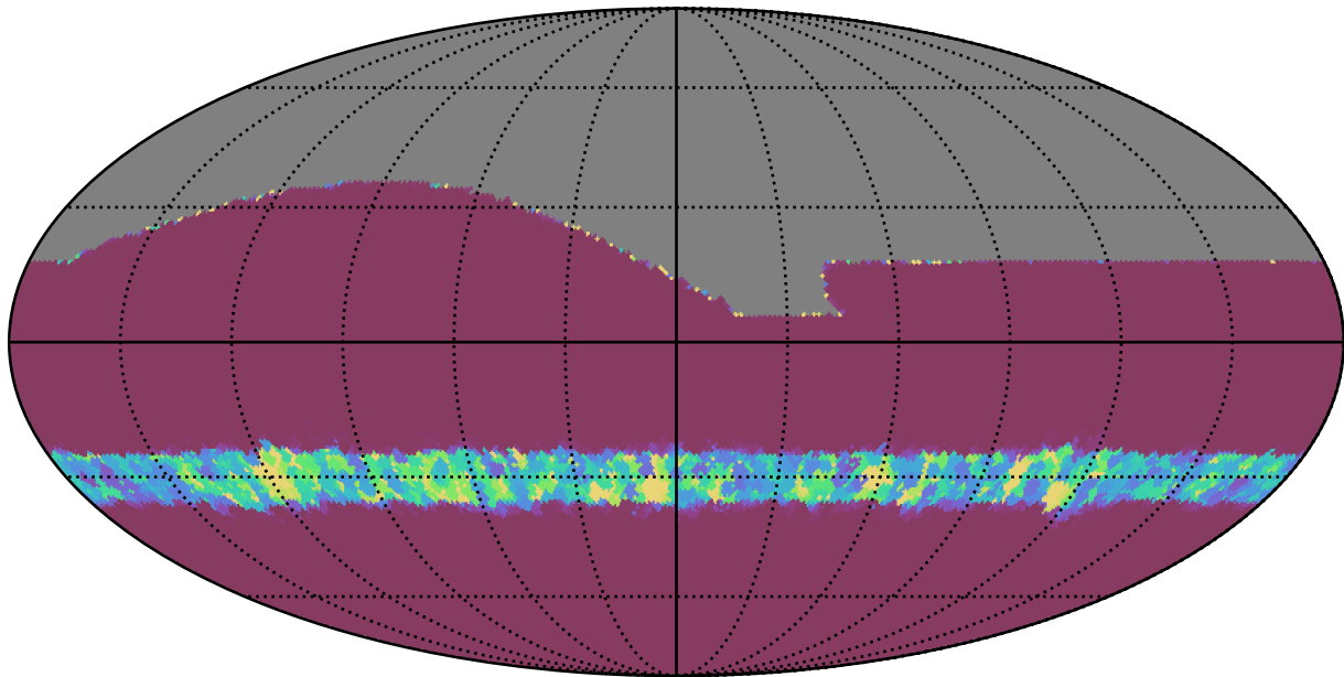
baseline_v2.0_10yrs All sky all bands: Min normairmass
