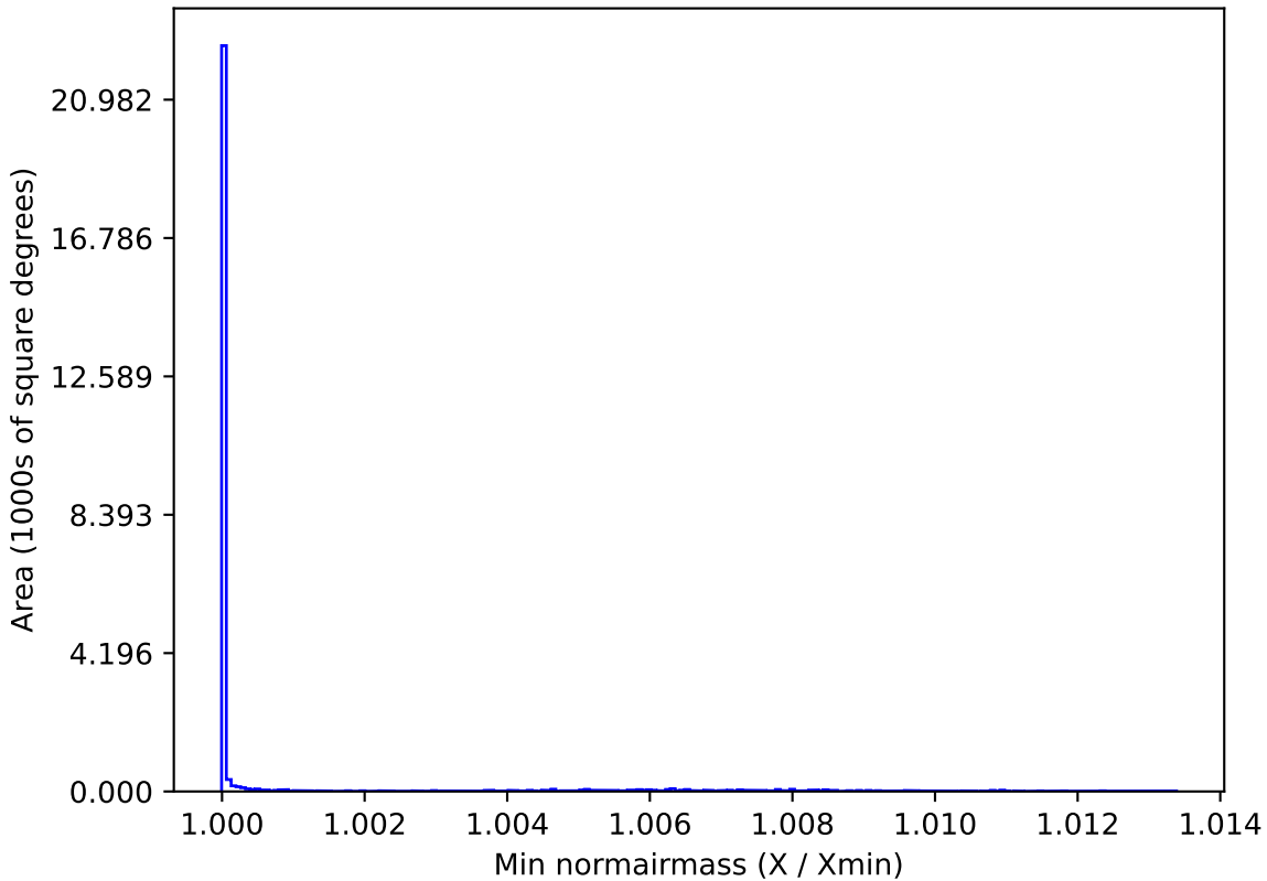
baseline_v2.0_10yrs All sky all bands: Min normairmass
