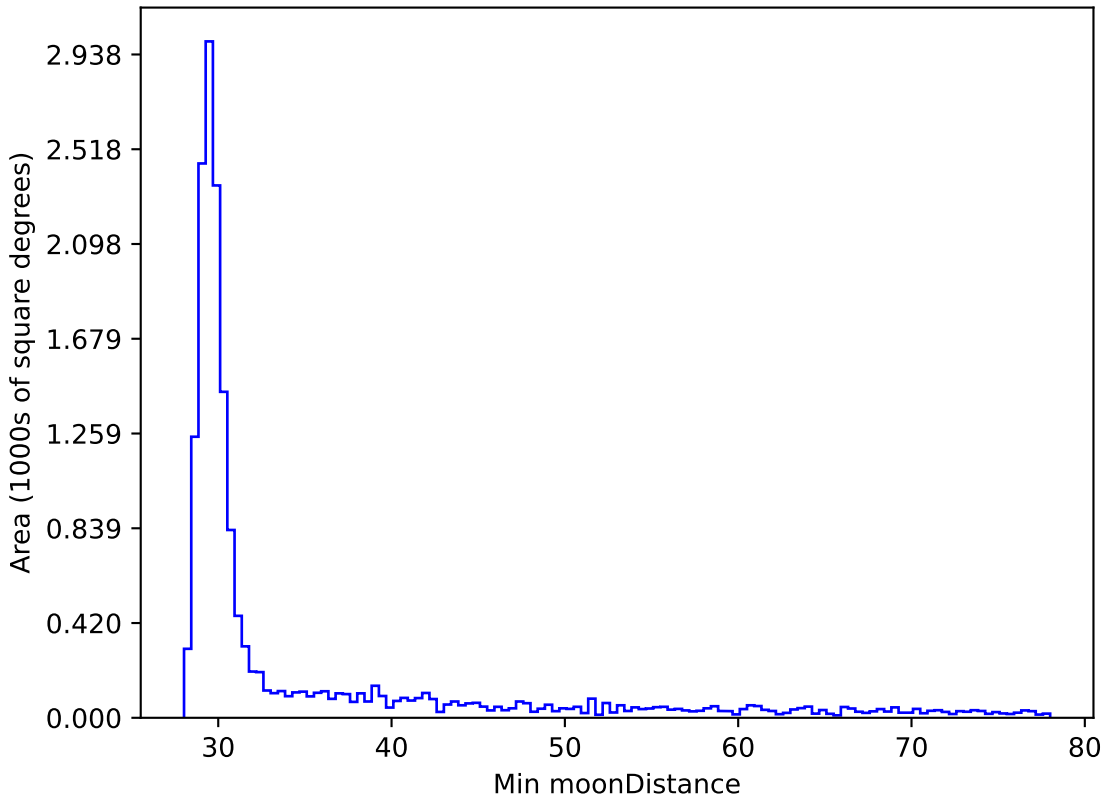
baseline_v2.0_10yrs WFD z band: Min moonDistance
