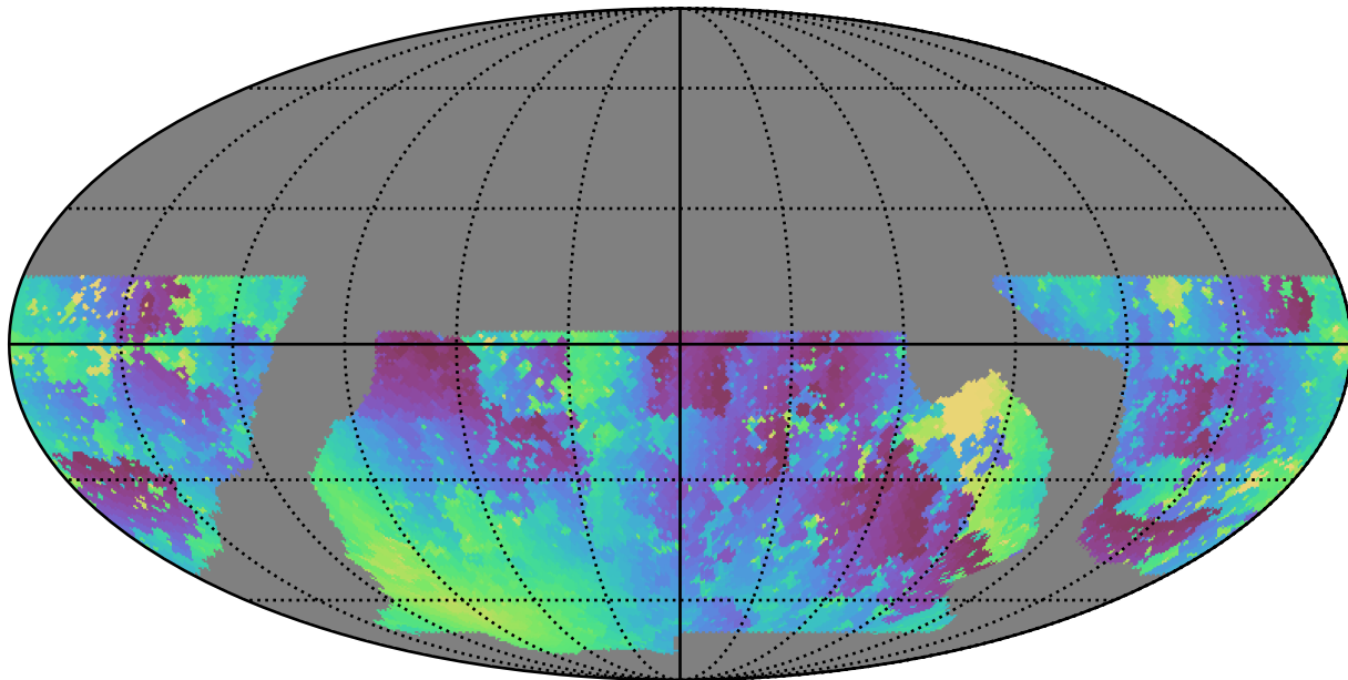
baseline_v2.0_10yrs WFD u band: Min moonDistance
