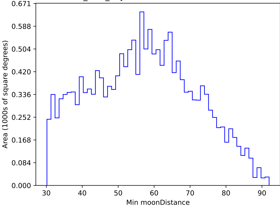
baseline_v2.0_10yrs WFD u band: Min moonDistance
