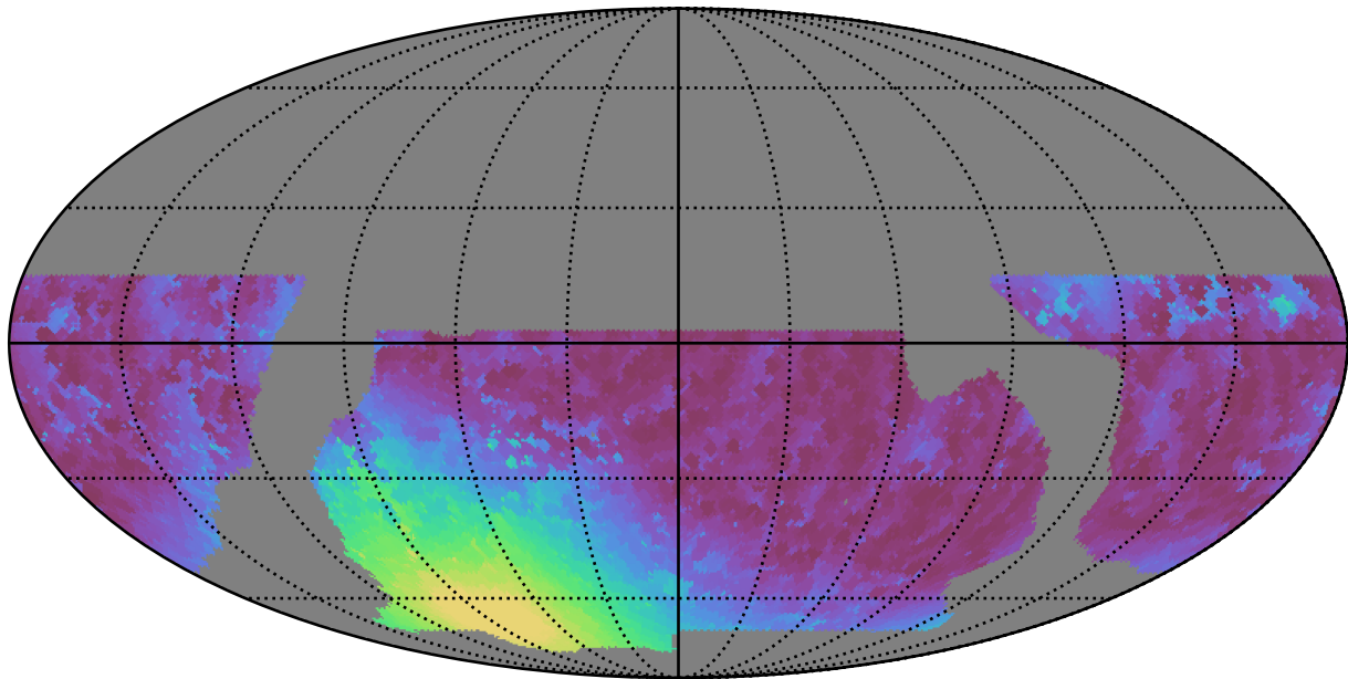
baseline_v2.0_10yrs WFD r band: Min moonDistance
