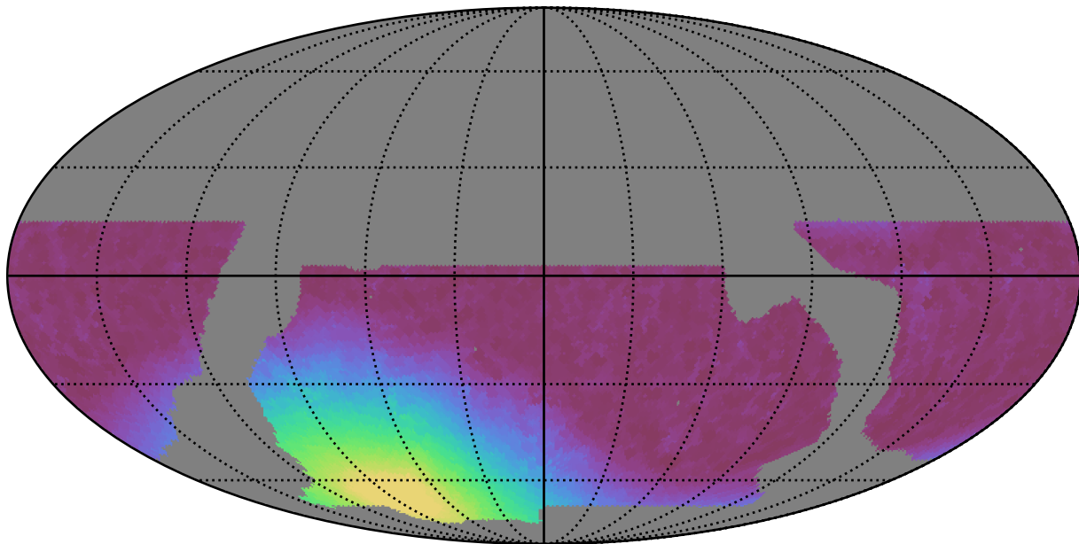
baseline_v2.0_10yrs WFD i band: Min moonDistance
