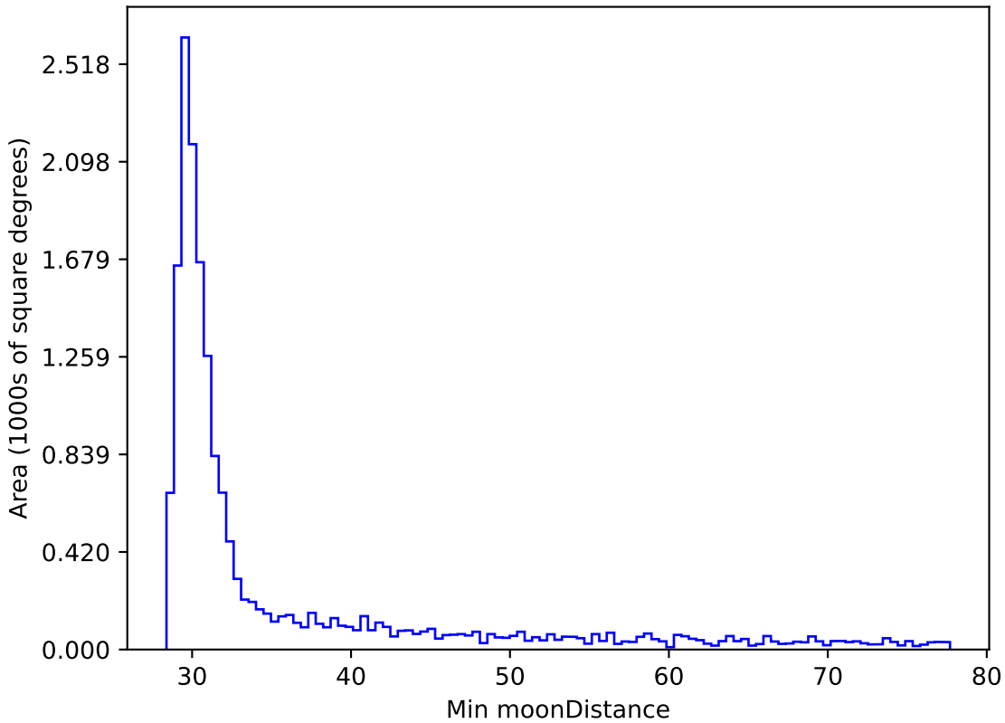
baseline_v2.0_10yrs WFD i band: Min moonDistance
