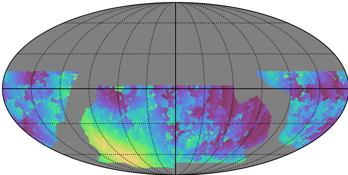
baseline_v2.0_10yrs WFD g band: Min moonDistance
