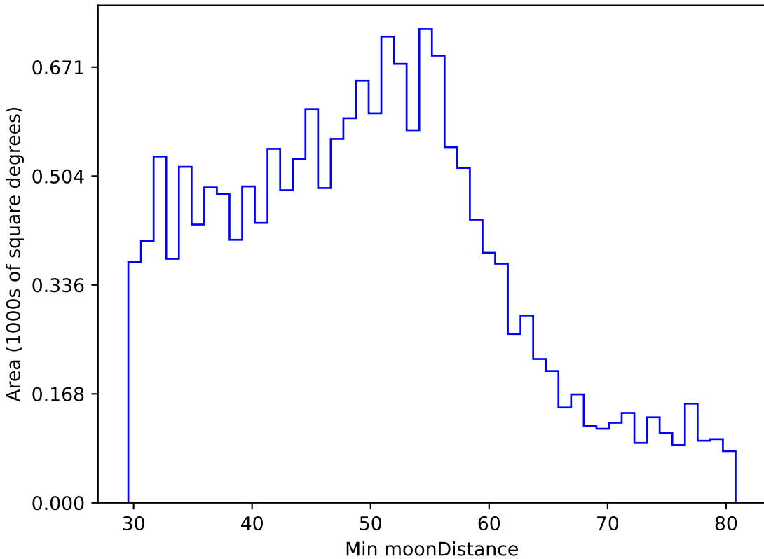
baseline_v2.0_10yrs WFD g band: Min moonDistance
