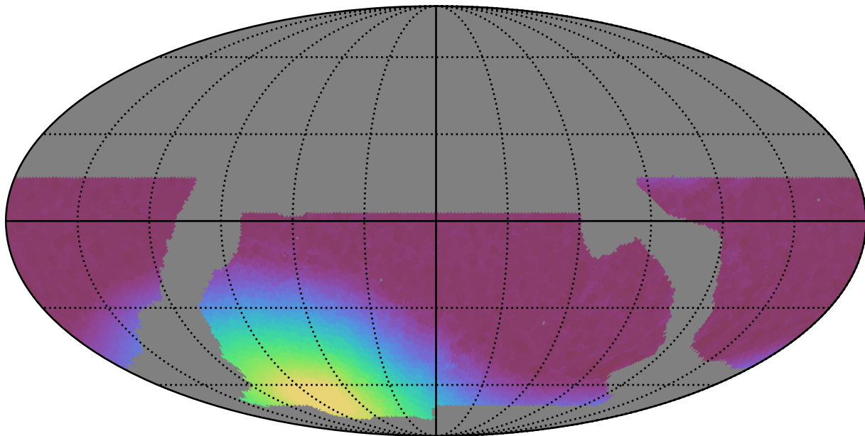
baseline_v2.0_10yrs WFD all bands: Min moonDistance
