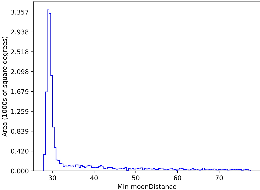
baseline_v2.0_10yrs WFD all bands: Min moonDistance
