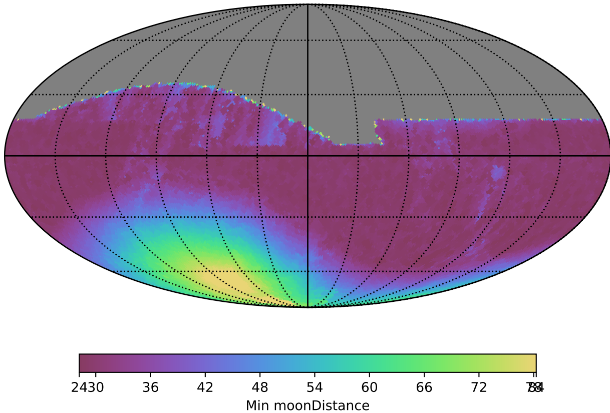
baseline_v2.0_10yrs All sky z band: Min moonDistance
