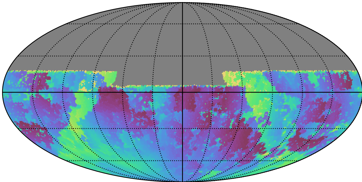
baseline_v2.0_10yrs All sky u band: Min moonDistance
