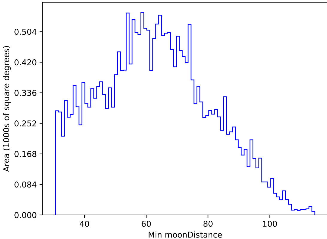
baseline_v2.0_10yrs All sky u band: Min moonDistance
