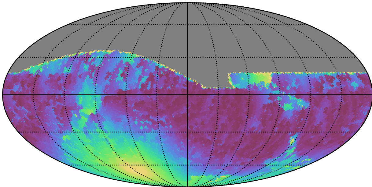
baseline_v2.0_10yrs All sky r band: Min moonDistance
