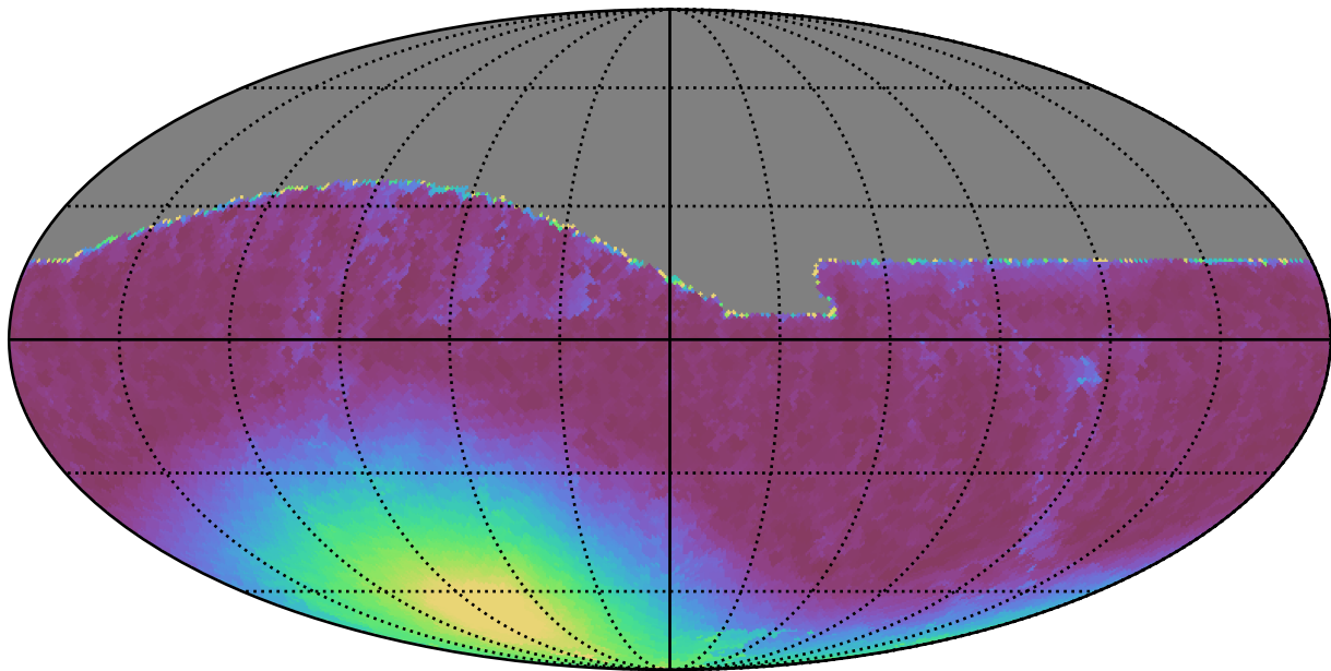
baseline_v2.0_10yrs All sky i band: Min moonDistance
