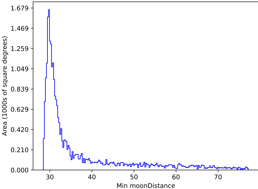
baseline_v2.0_10yrs All sky i band: Min moonDistance
