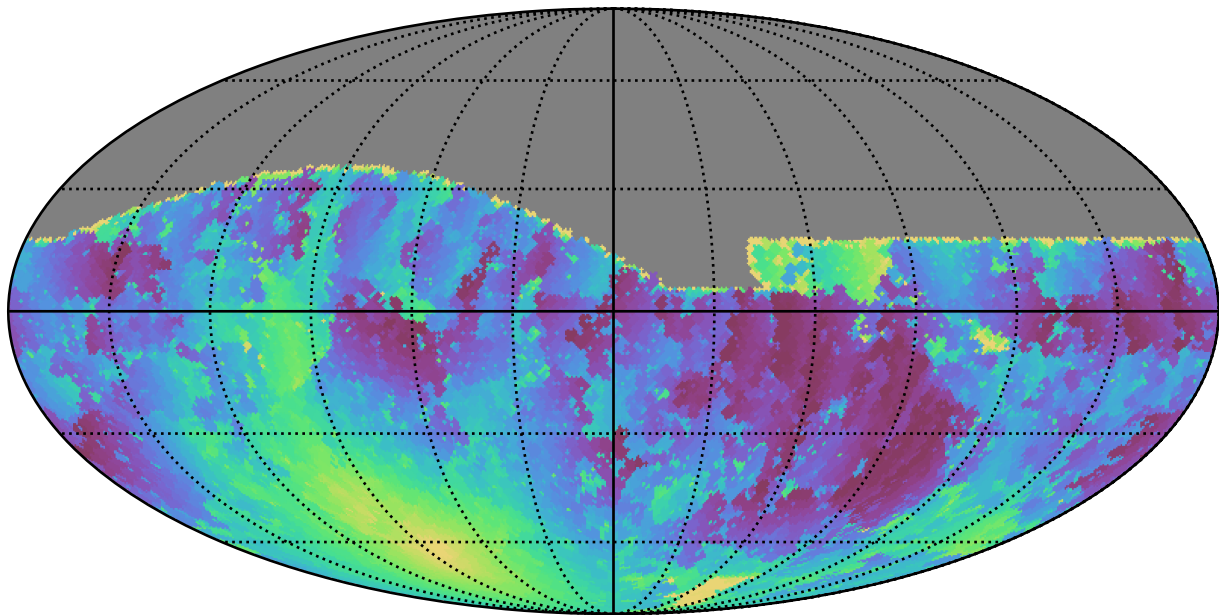
baseline_v2.0_10yrs All sky g band: Min moonDistance
