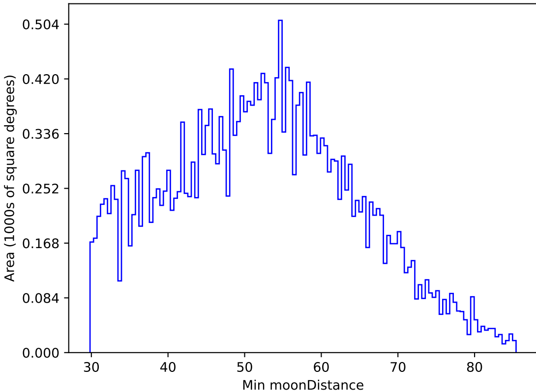
baseline_v2.0_10yrs All sky g band: Min moonDistance
