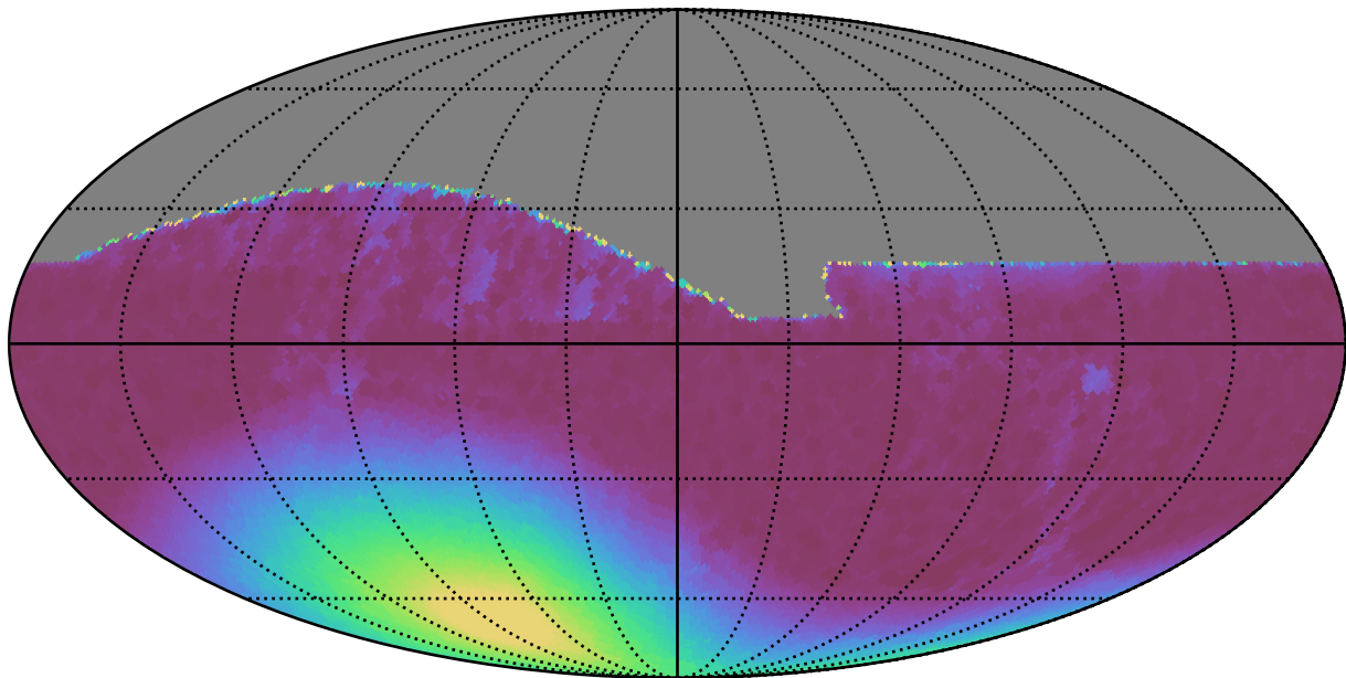
baseline_v2.0_10yrs All sky all bands: Min moonDistance
