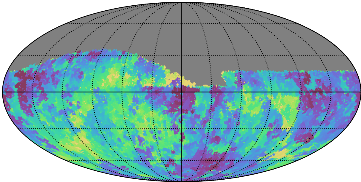
baseline_v2.0_10yrs Yr 1 z band: Min fiveSigmaDepth
