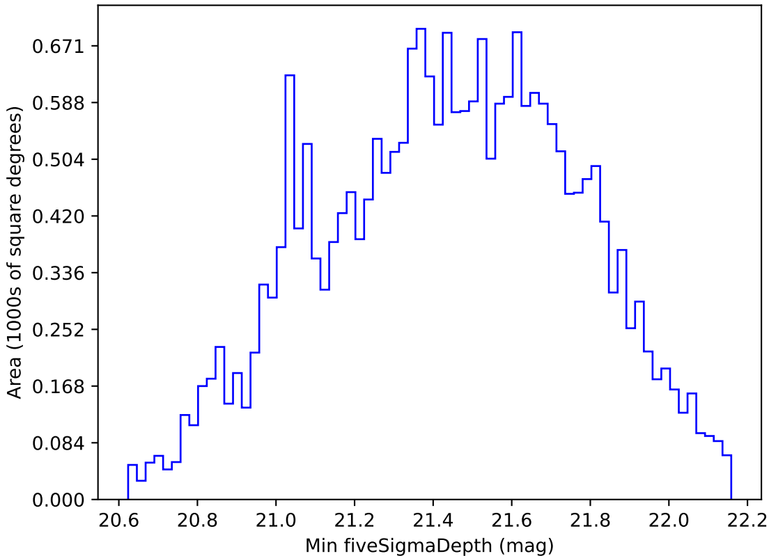
baseline_v2.0_10yrs Yr 1 y band: Min fiveSigmaDepth
