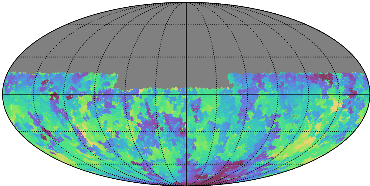
baseline_v2.0_10yrs Yr 1 u band: Min fiveSigmaDepth
