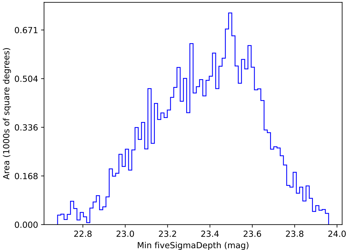
baseline_v2.0_10yrs Yr 1 u band: Min fiveSigmaDepth
