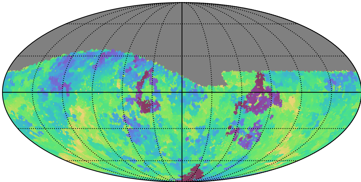
baseline_v2.0_10yrs Yr 1 r band: Min fiveSigmaDepth
