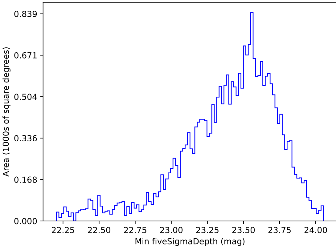
baseline_v2.0_10yrs Yr 1 r band: Min fiveSigmaDepth
