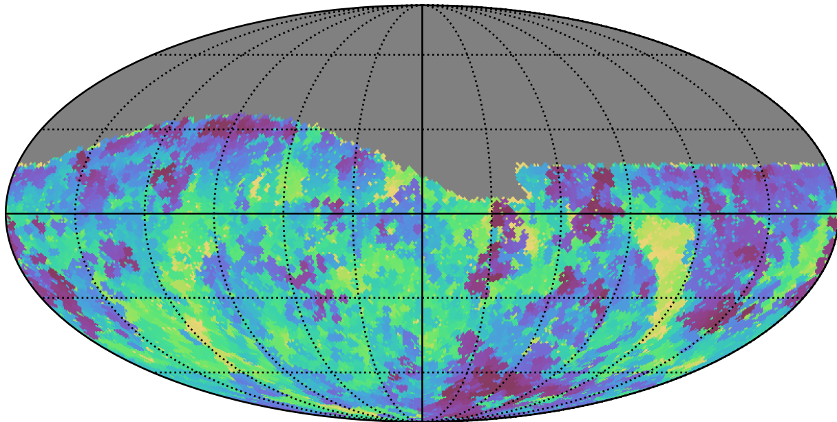
baseline_v2.0_10yrs Yr 1 i band: Min fiveSigmaDepth
