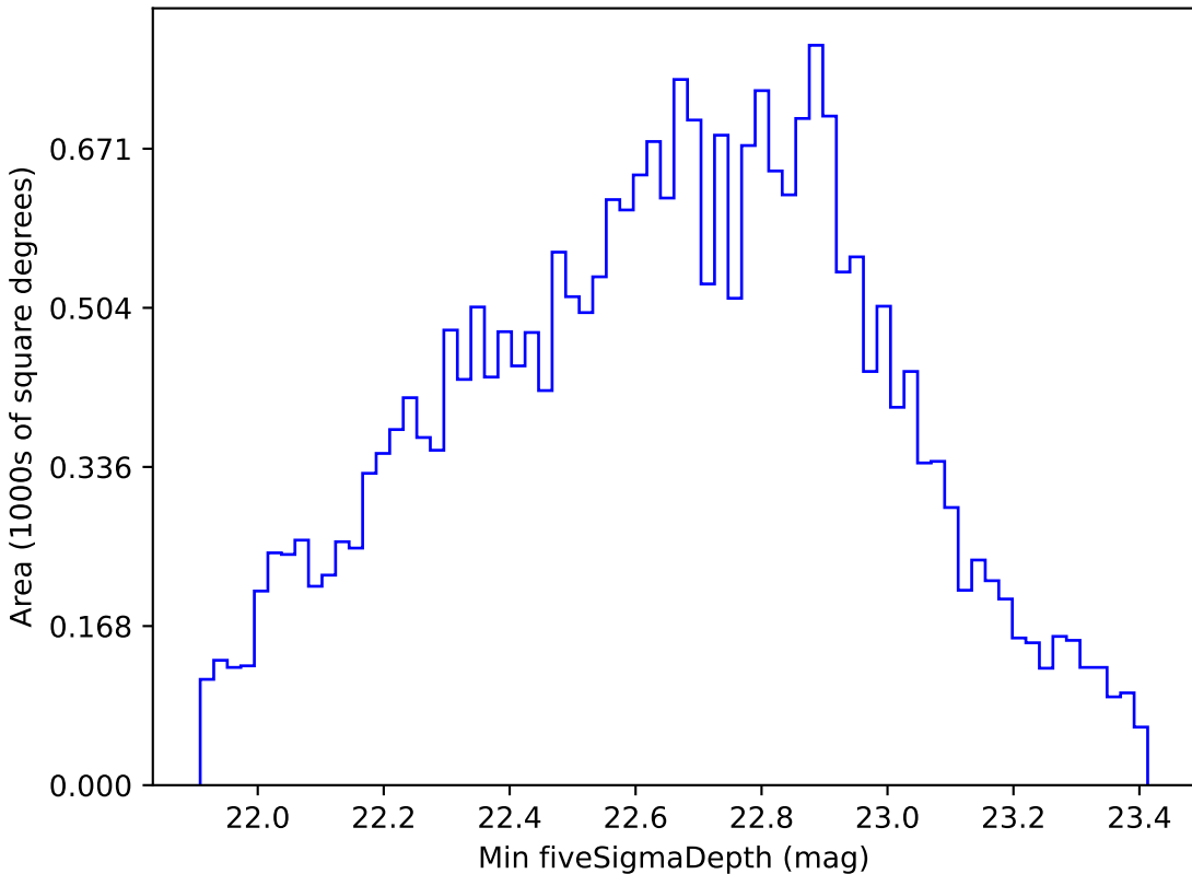
baseline_v2.0_10yrs Yr 1 i band: Min fiveSigmaDepth
