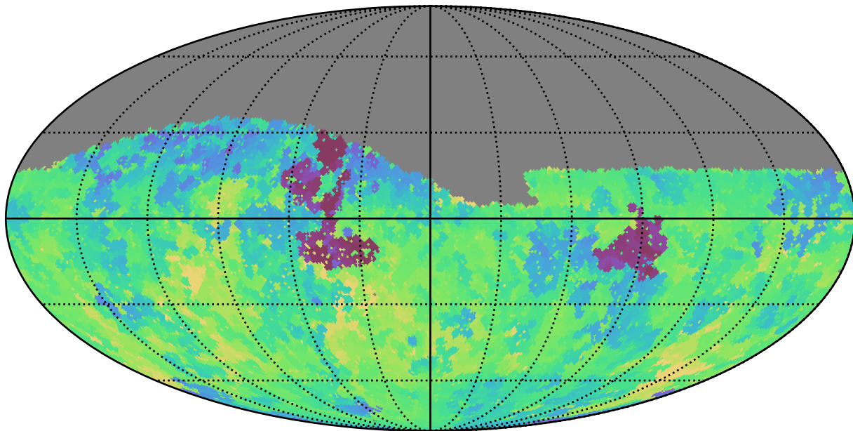
baseline_v2.0_10yrs Yr 1 g band: Min fiveSigmaDepth
