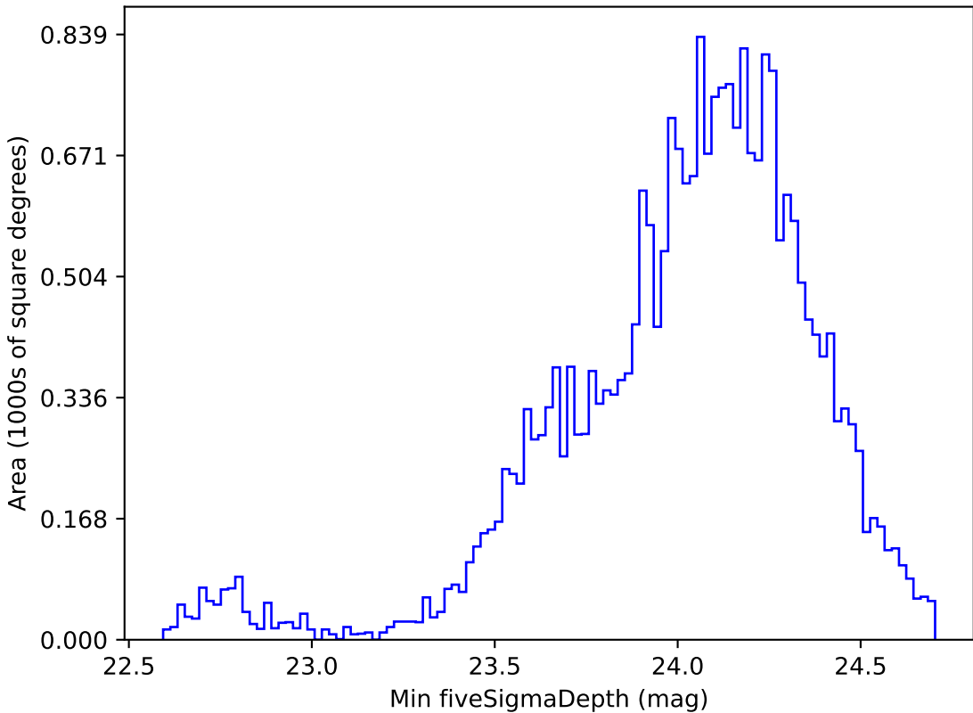
baseline_v2.0_10yrs Yr 1 g band: Min fiveSigmaDepth
