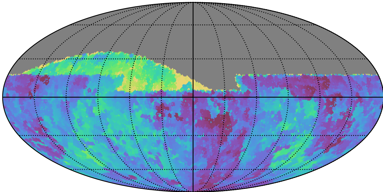
baseline_v2.0_10yrs Yr 1 all bands: Min fiveSigmaDepth
