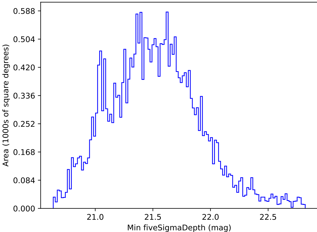
baseline_v2.0_10yrs Yr 1 all bands: Min fiveSigmaDepth
