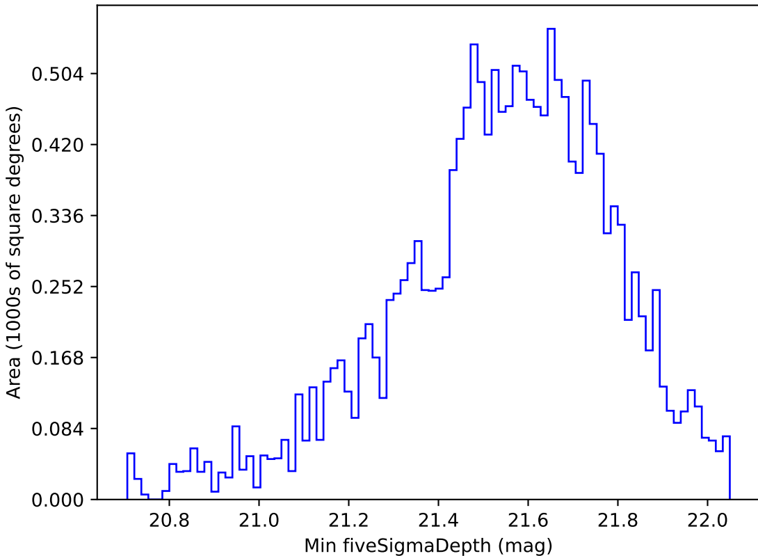
baseline_v2.0_10yrs WFD z band: Min fiveSigmaDepth
