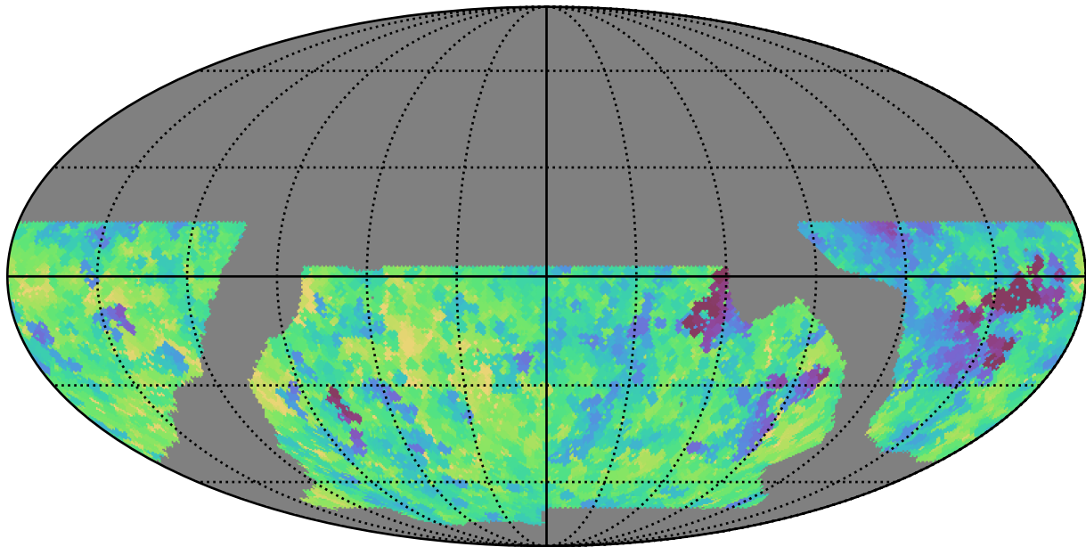
baseline_v2.0_10yrs WFD y band: Min fiveSigmaDepth
