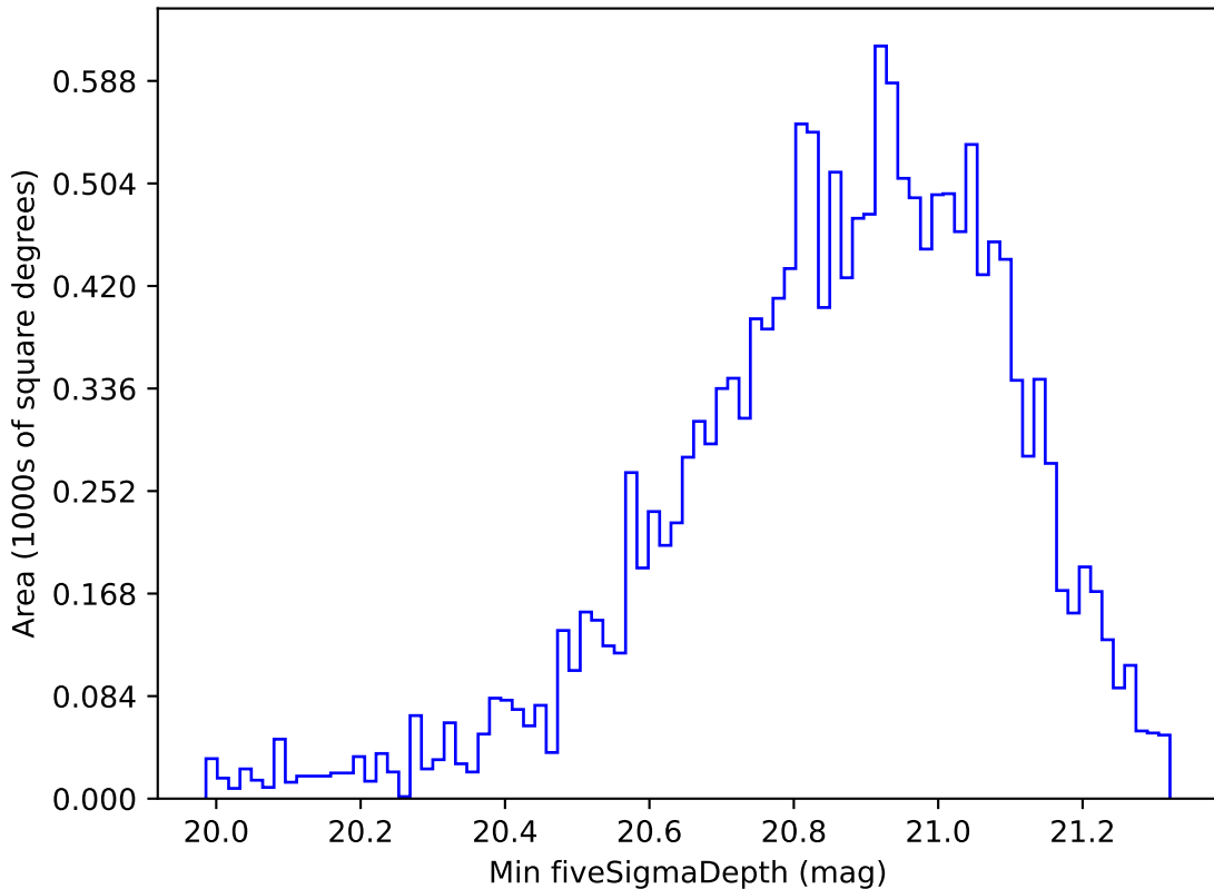
baseline_v2.0_10yrs WFD y band: Min fiveSigmaDepth
