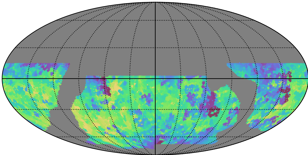
baseline_v2.0_10yrs WFD u band: Min fiveSigmaDepth
