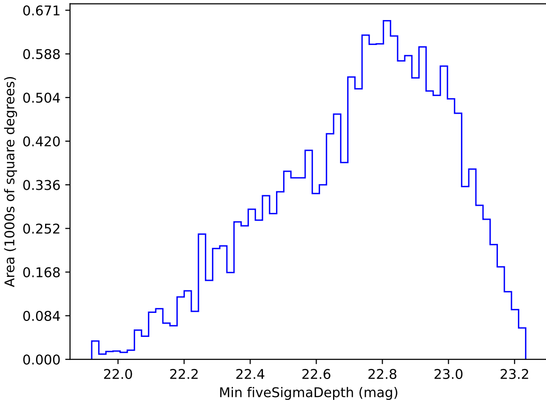
baseline_v2.0_10yrs WFD u band: Min fiveSigmaDepth
