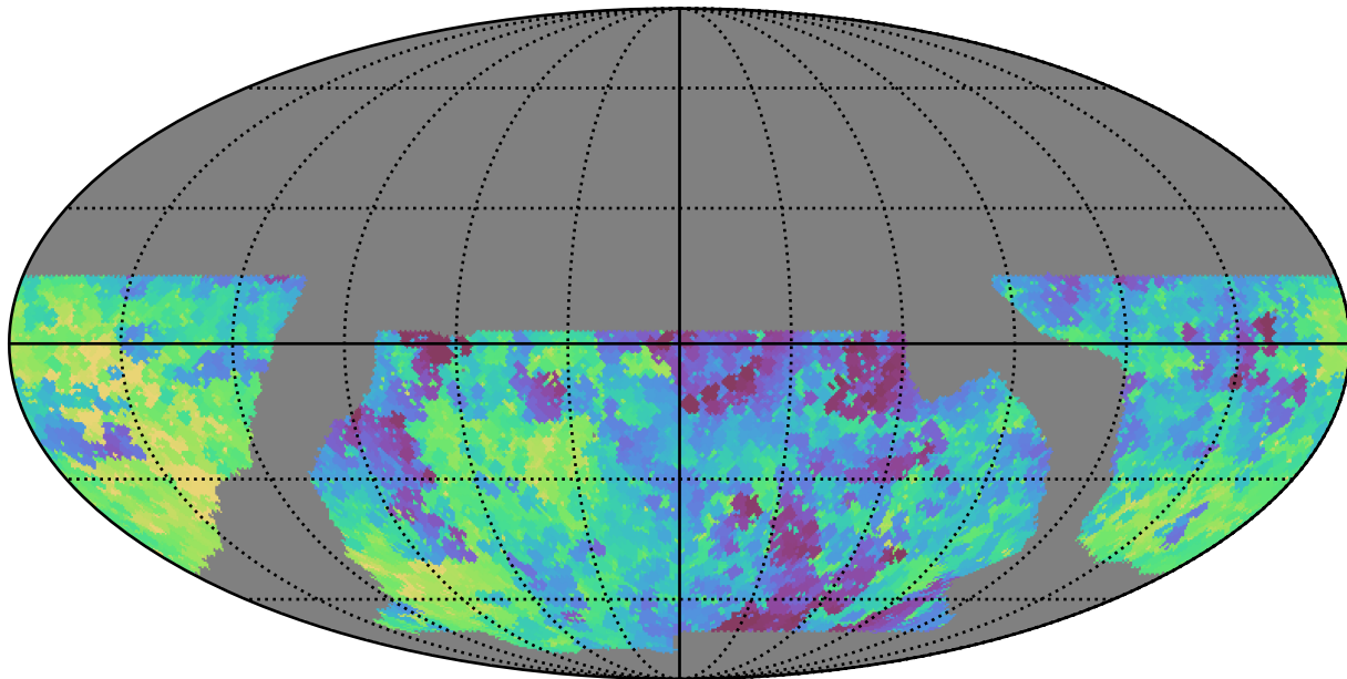
baseline_v2.0_10yrs WFD r band: Min fiveSigmaDepth
