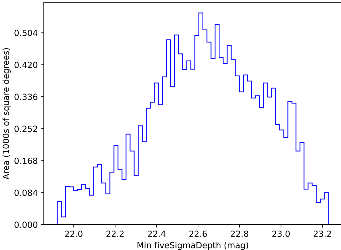
baseline_v2.0_10yrs WFD r band: Min fiveSigmaDepth
