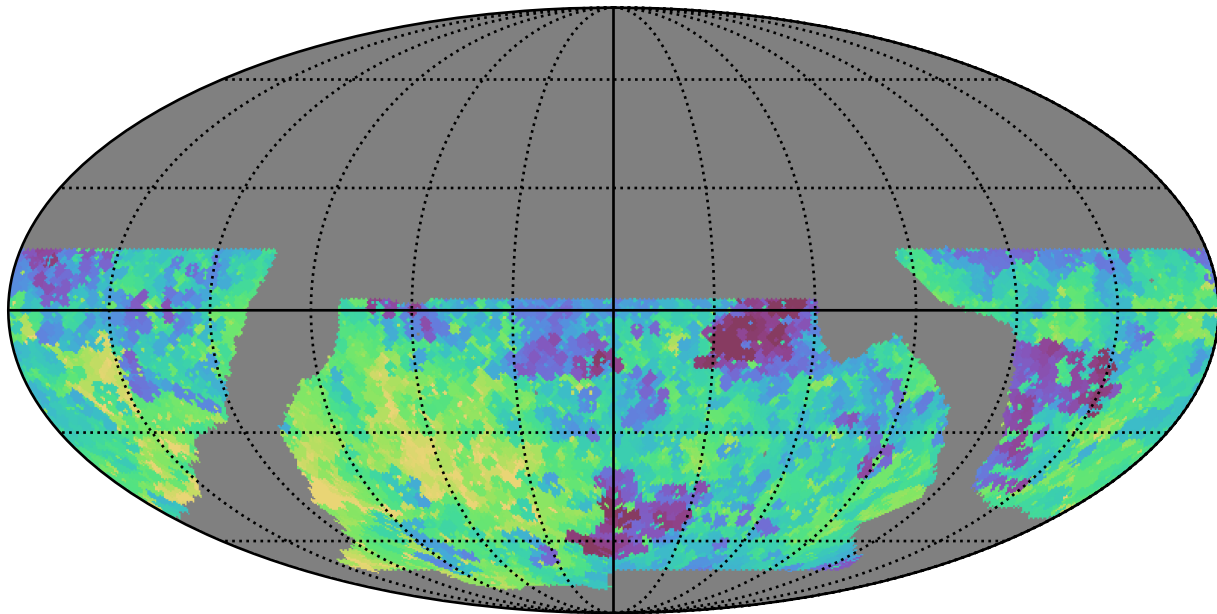
baseline_v2.0_10yrs WFD i band: Min fiveSigmaDepth
