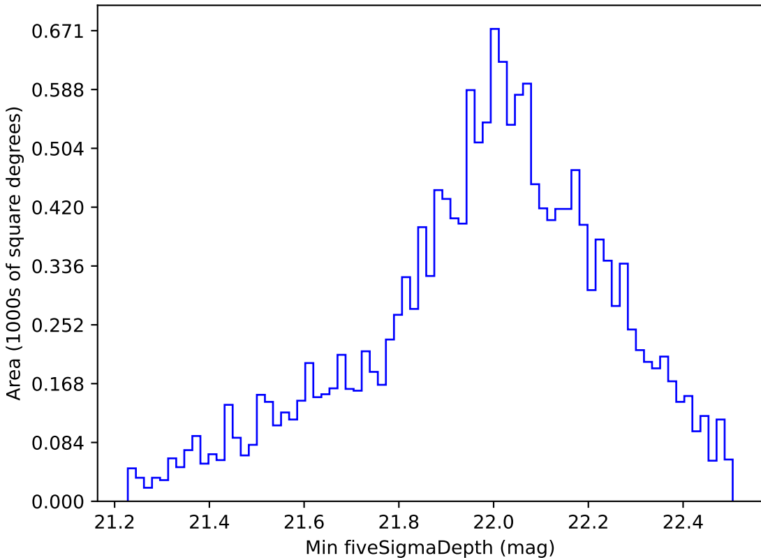
baseline_v2.0_10yrs WFD i band: Min fiveSigmaDepth
