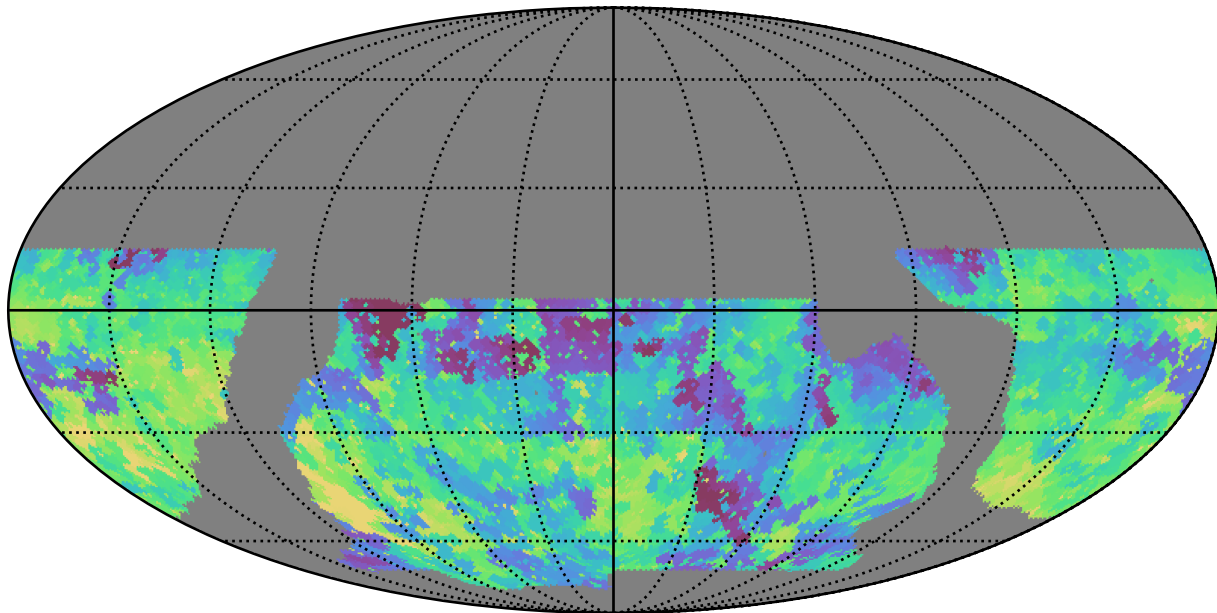
baseline_v2.0_10yrs WFD g band: Min fiveSigmaDepth
