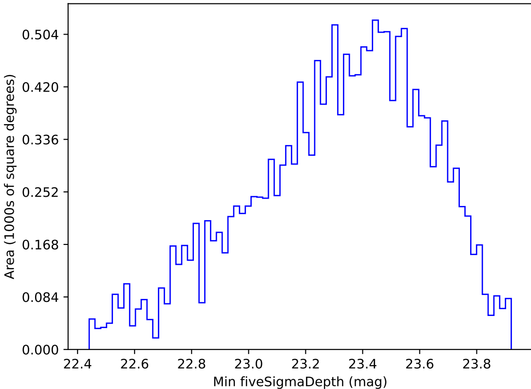
baseline_v2.0_10yrs WFD g band: Min fiveSigmaDepth
