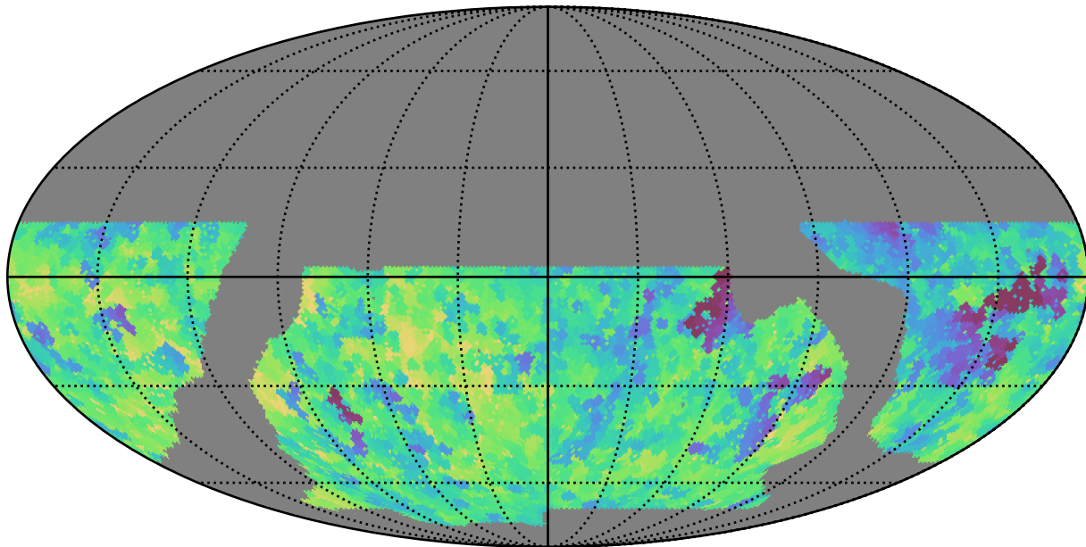
baseline_v2.0_10yrs WFD all bands: Min fiveSigmaDepth
