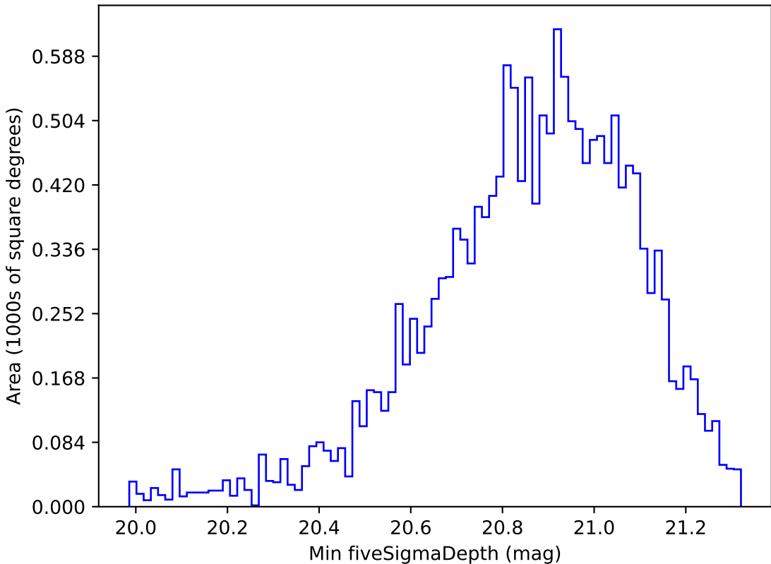
baseline_v2.0_10yrs WFD all bands: Min fiveSigmaDepth
