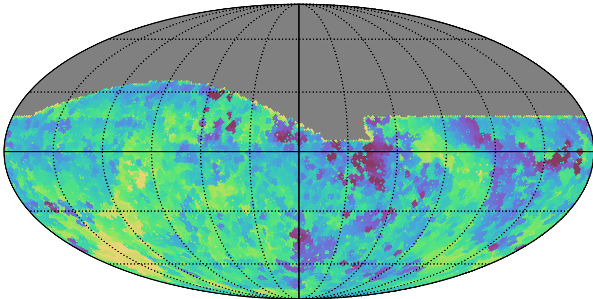
baseline_v2.0_10yrs All sky z band: Min fiveSigmaDepth
