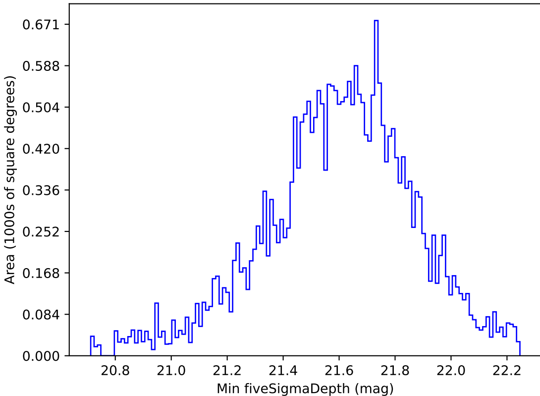
baseline_v2.0_10yrs All sky z band: Min fiveSigmaDepth
